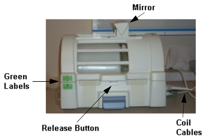
Figure 3-2 Split Head Coil
